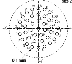
20-41 41 contacts size 20
